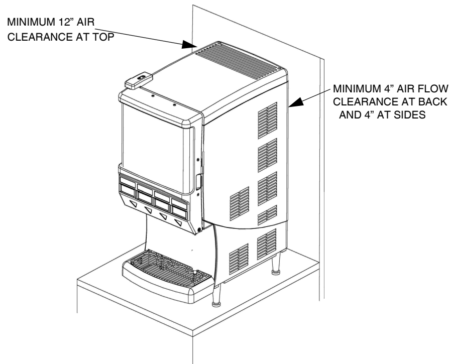
Figure 4. Minimum Clearances
