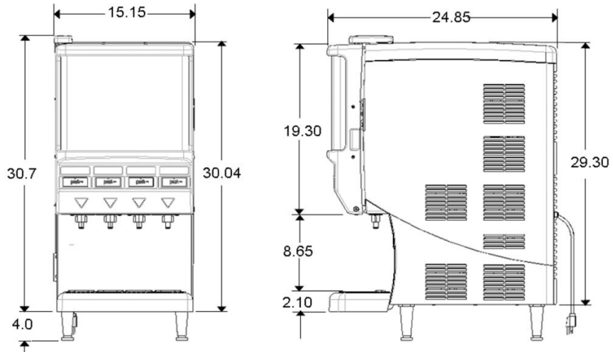
Figure 1. Quest Elite 4000
