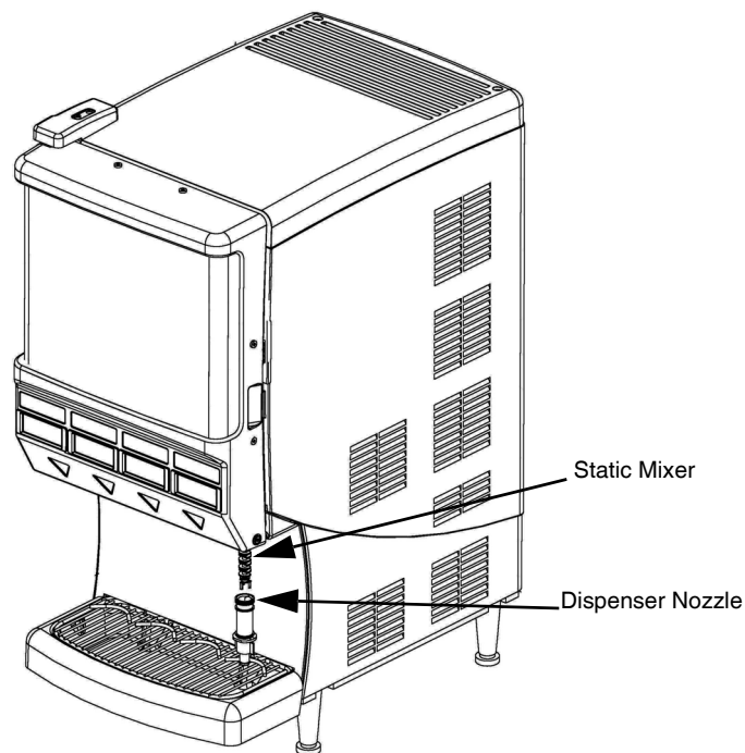
Figure 8. Dispense Nozzle
