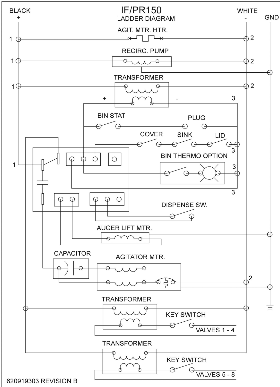
Figure 8. Ladder Diagram
