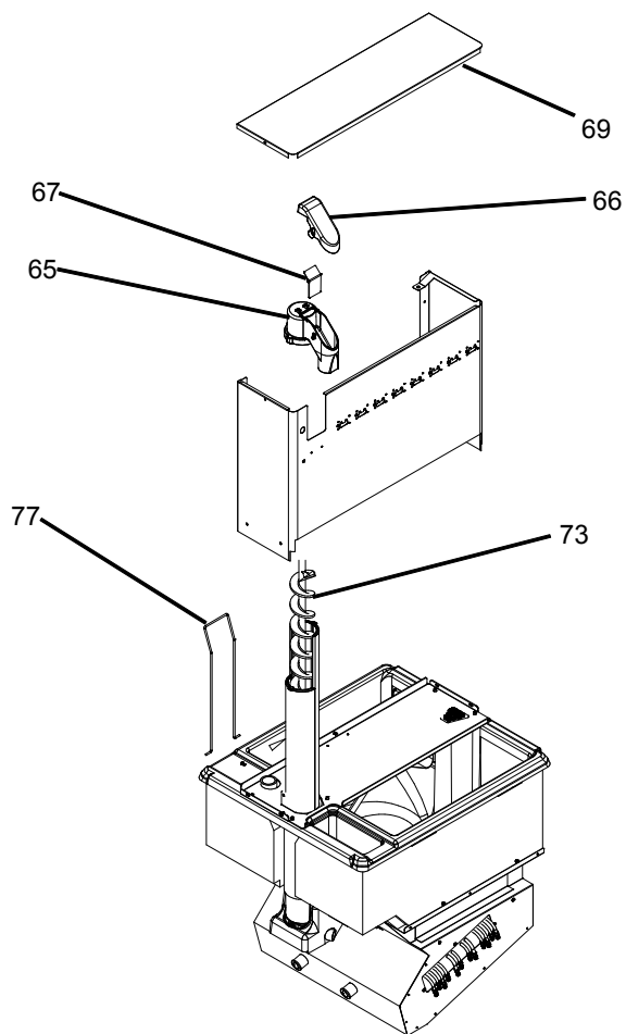
Figure 4. Auger Assembly
