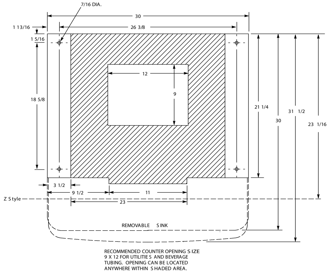
Figure 2. IDC 2XX Mounting Template
