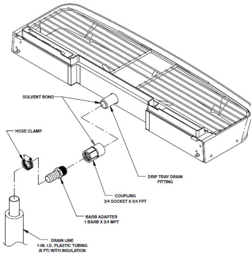
Figure 4. Drip Tray Drain Assembly
