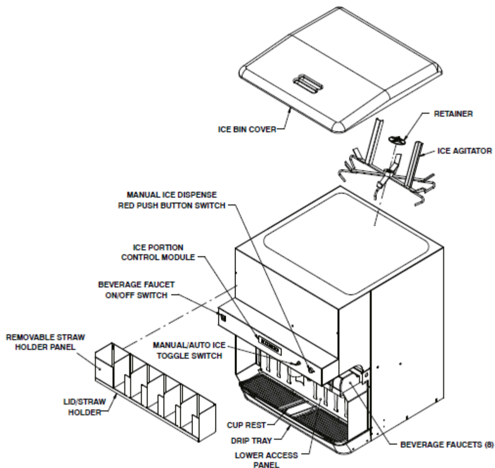
Figure 1. Parts Identification
