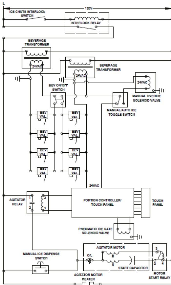
Figure 8. Wiring Schematic (115 Volt)
