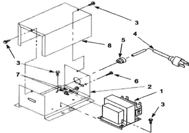
Figure 2. Alta 1522 Transformer Assembly
