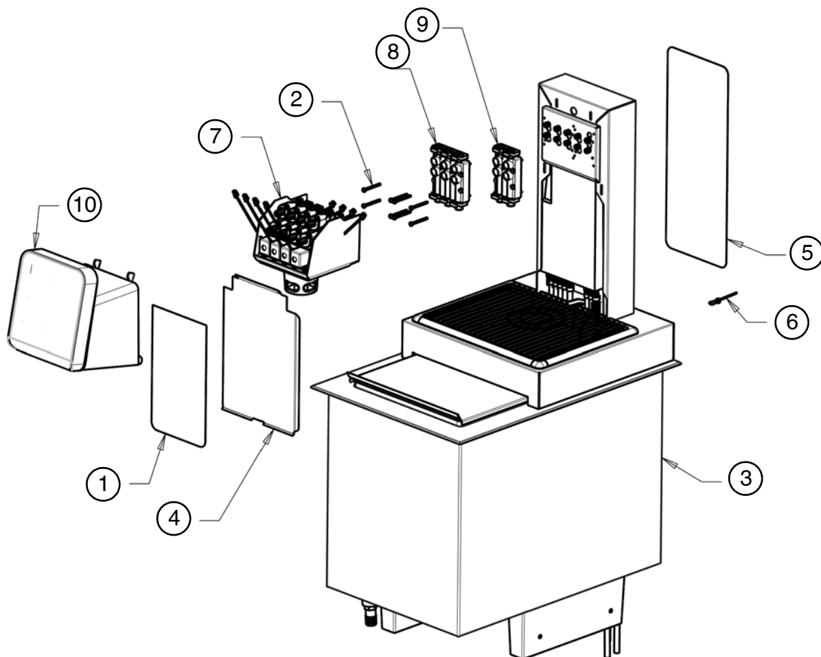
Figure 1. Alta 1522 Tower Assembly
